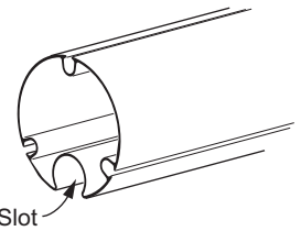
Roller Tube w/ Utility Slot
